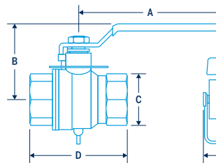
NPT Model: BD075N thru BD200N
