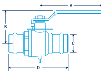
Press Model: BD075P thru BD200P
