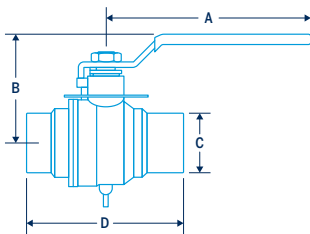
Sweat Model: BD075S thru BD200S
